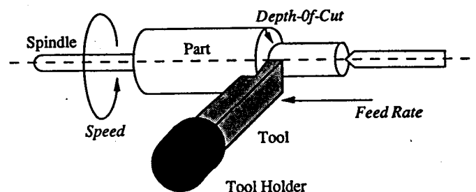
Figure 2 Parameters of a Typical Turning Operation
